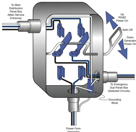
Figure 1. DPDT Transfer Switch
